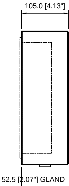
RIGHT SIDE VIEW PANEL PC SHOWN PHANTOM
