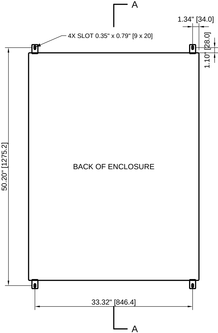
REAR VIEW WALL-MOUNT HOLE PATTERN
