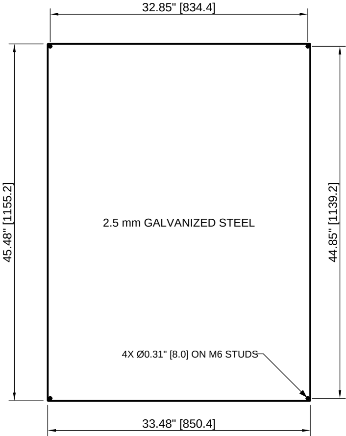
MOUNTING PANEL REMOVABLE
