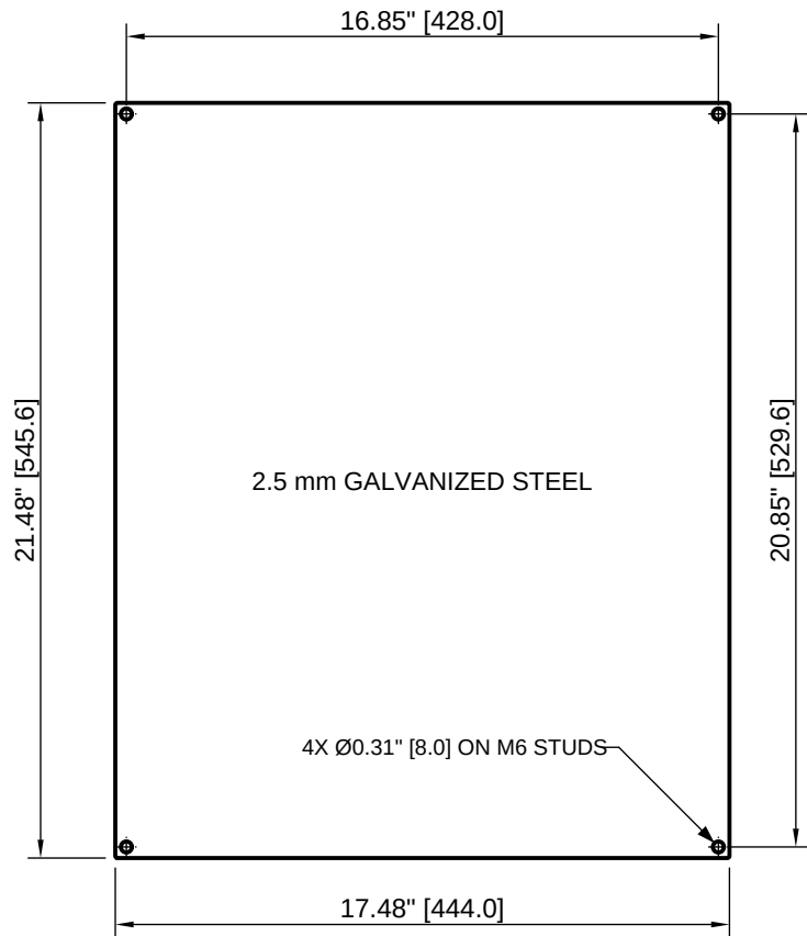
MOUNTING PANEL REMOVABLE
