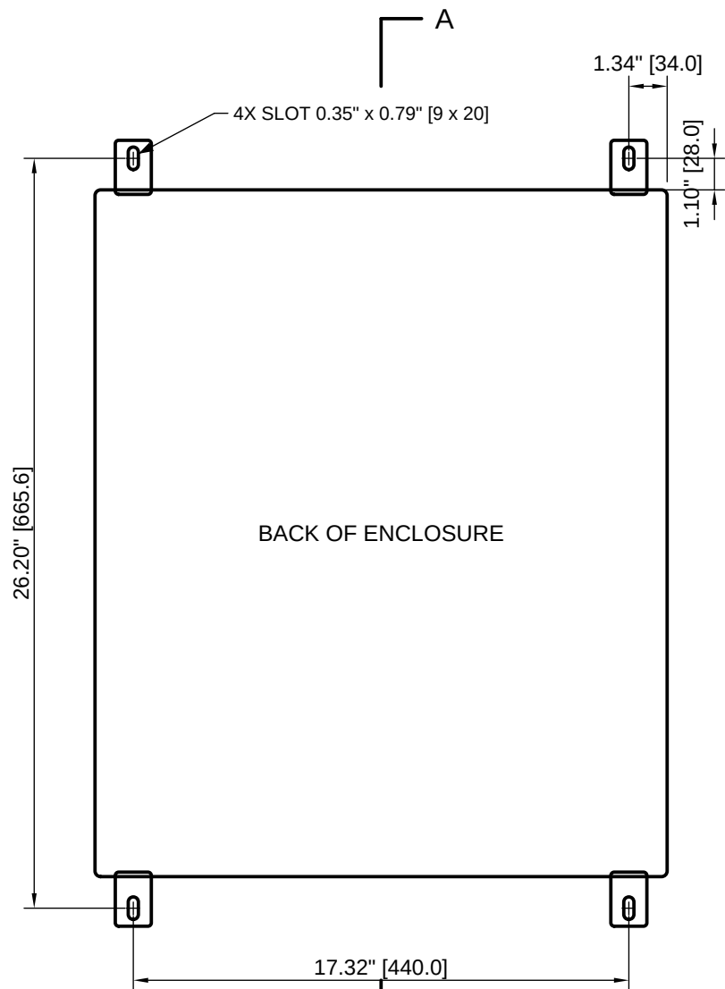
REAR VIEW WALL-MOUNT HOLE PATTERN
