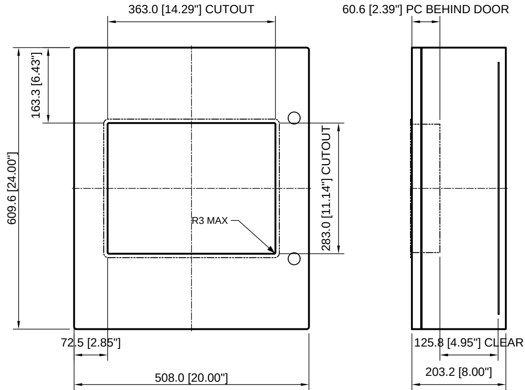
DOOR - OUTSIDE VIEW CUTOUT CENTRED ON THE DOOR
