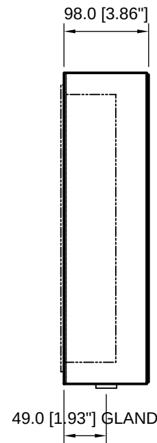
RIGHT SIDE VIEW PANEL PC SHOWN PHANTOM
