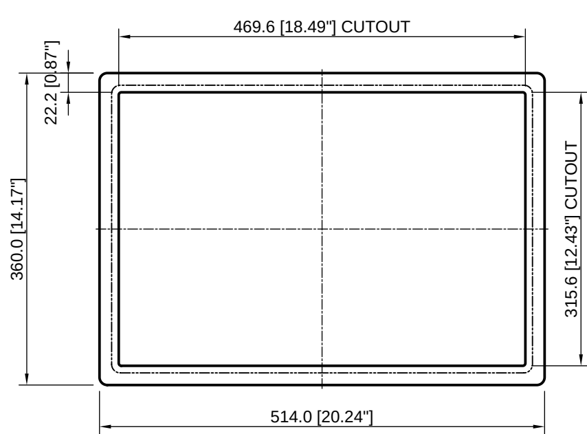
FRONT VIEW DISPLAY SHOWN PHANTOM
