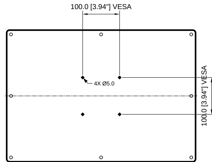
REAR VIEW REMOVABLE COVER, 8 SCREWS
